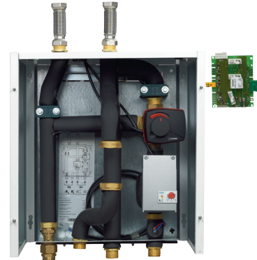
Kit 2 zones PAC 1 service
