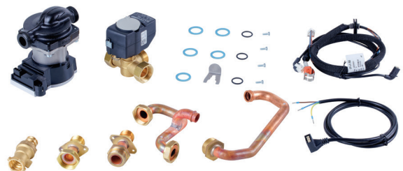
Kit 2 zones Ixtra M
